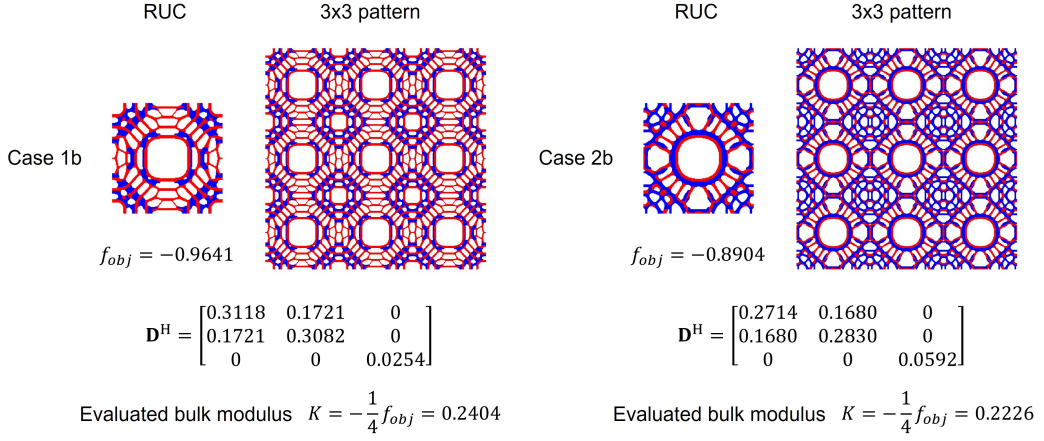
Fig. 3. Three-phase designs for maximized bulk modulus
