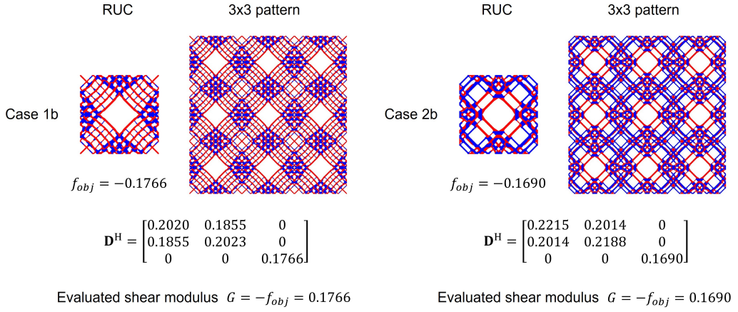
Fig. 4. Three-phase designs for maximized shear modulus
