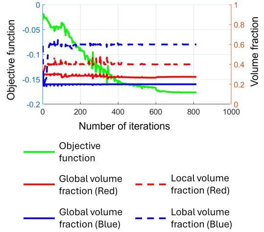
Fig. 7. History curves for Case 1b of maximized shear modulus
