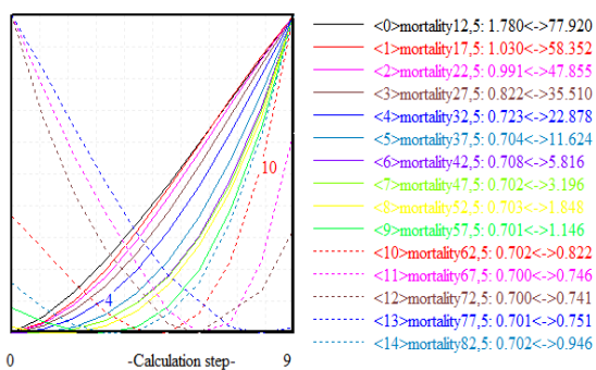
Figure 11. Time graph drawn for the variables of “mortality” (number of died trees) with individual scale
