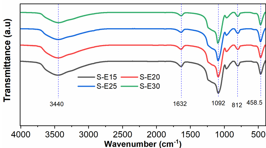
Figure 5. FTIR spectra of the synthesized SiO 2 samples
