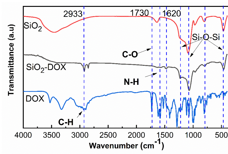
Figure 9. FTIR spectra of pure DOX and the S-E25 sample before and after drug loading experiment.
