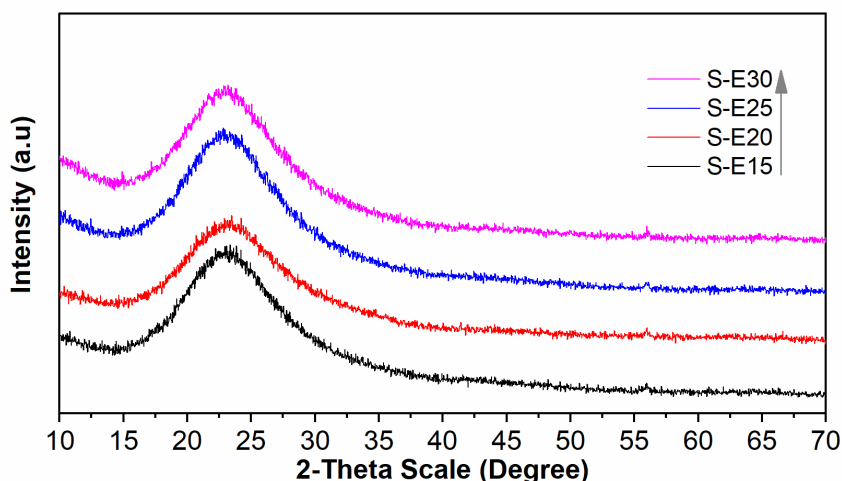
Figure 4. XRD patterns of the SiO 2 nanoparticles
