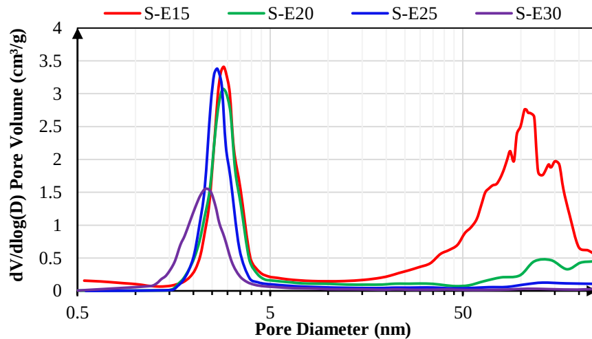
Figure 7. Diagram of pore size distribution of \text{SiO}_2 nanoparticles
