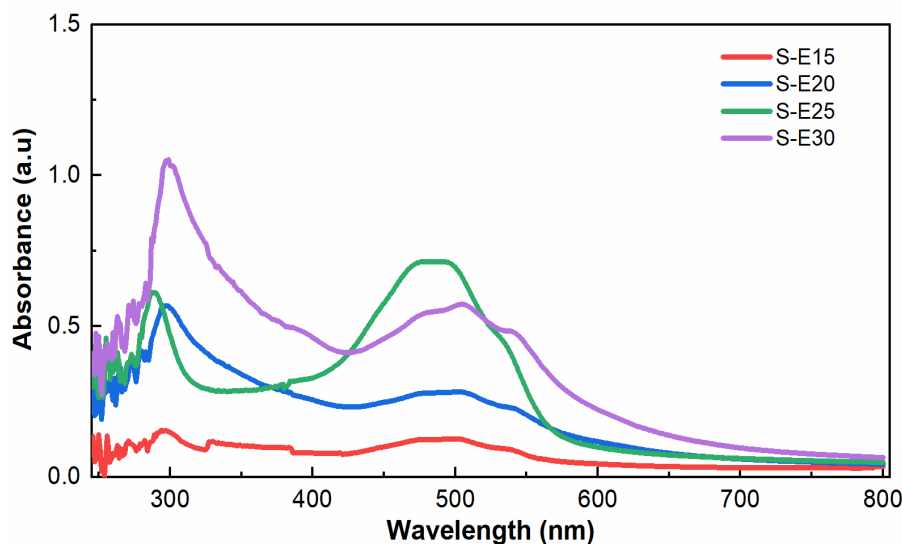
Figure 8. The UV-vis spectra of the free DOX in the solution after the drug loading experiment for the \text{SiO}_2 samples.
