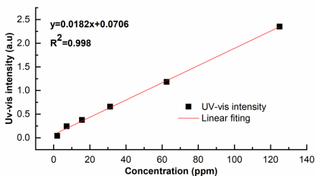
Figure 1. The calibration curve of relationship between the UV-vis intensity and DOX concentration
