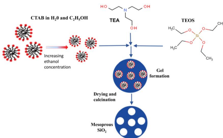
Figure 3. Schematic illustration of the formation of mesoporous \text{SiO}_2 nanoparticles.
