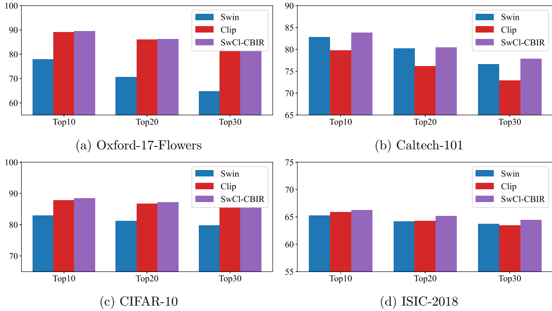
Figure 7: Illustration of the SwCl-CBIR model performance on the datasets
