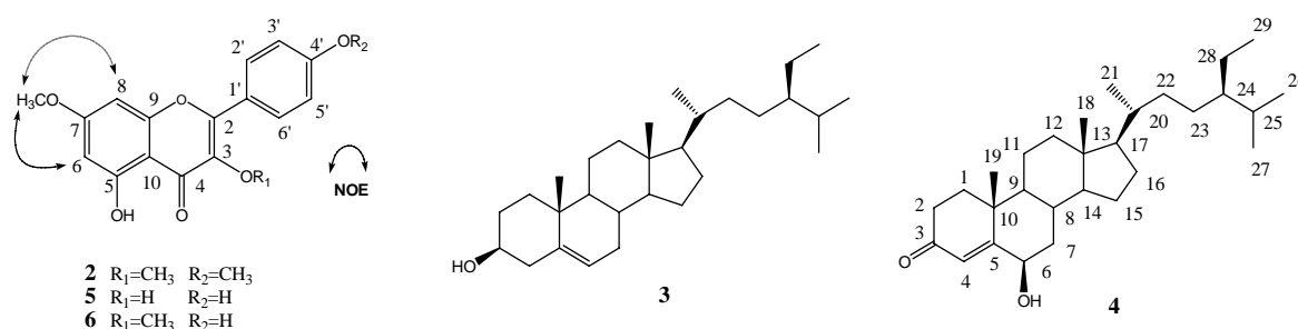
Figure 1: Chemical structures of the isolates 2-6 and diagnostic NOESY interactions of 5 and 6
