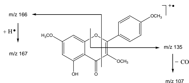
Figure 2: Diagnostic EI-MS fragmentations of 2
