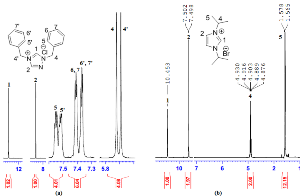
Figure 2: ^1\text{H} NMR spectra of M3 (a) and M4 (b)
