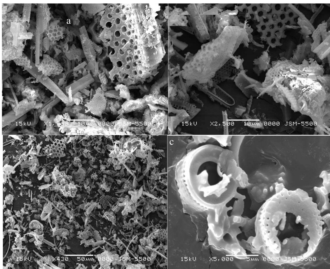
Figure 5. SEM images of the diatomite calcined at different temperatures: (a) – 900 °C; (b) – 1000 °C; (c) – 1100 °C; (d) – 1250 °C
