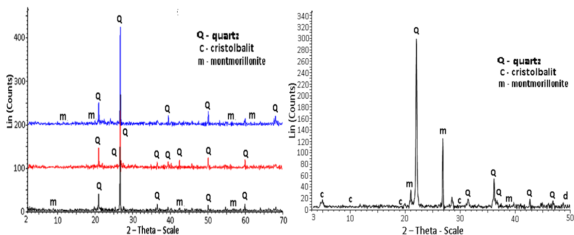
Figure 4. XRD of filter aids from Lam Dong diatomite: (a) – 900 °C; (b) – 1000 °C; (c) – 1100 °C; (d) – 1250 °C
