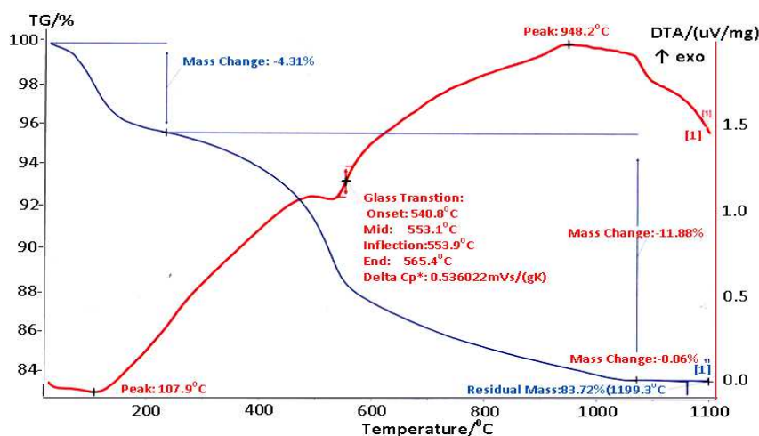
Fig. 1. The results of TG – DTA analysis of raw Lam dong diatomite
