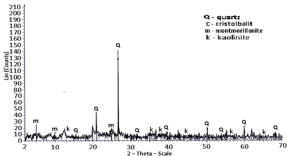
Figure 2. The XRD pattern of raw Lam Dong diatomite
