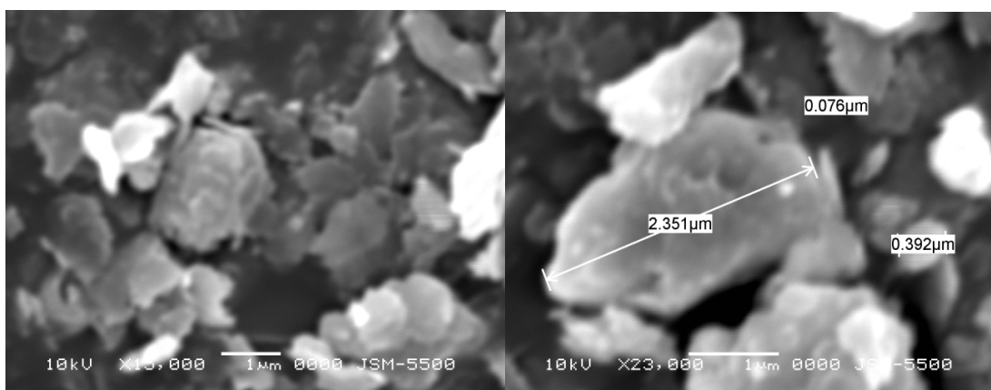
Figure 3. Scanning electron microscopes of raw Lam Dong diatomite
