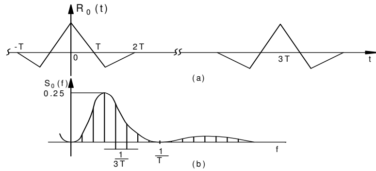
Figure 1a. Characteristics of NRZ bit periodical sequence 10110010
