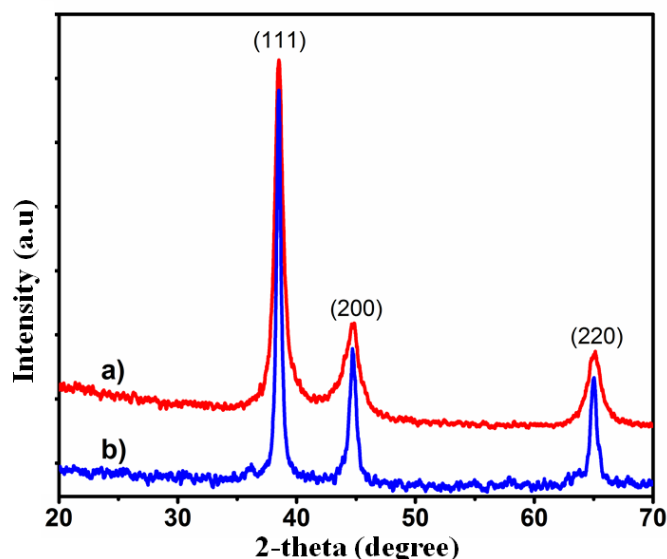
Figure 5. X-ray diffraction patterns of the spherical Ag NPs (a) and Ag nanorods (b).
