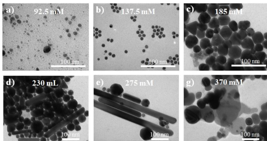
Figure 3. TEM images of Ag NPs at different concentrations of the reductant OCD-ol.
