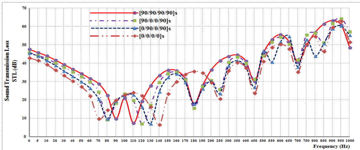
Figure 4. Influence of laminate configuration on STL of a simply supported double-composite plate with enclosed air cavity.
