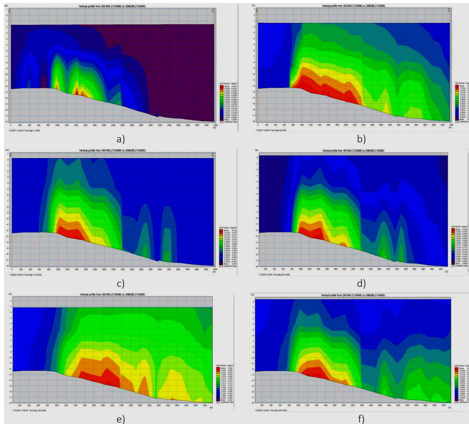
Figure 15. The distribution of sediment mud concentration with depth at cross-section MC01.
