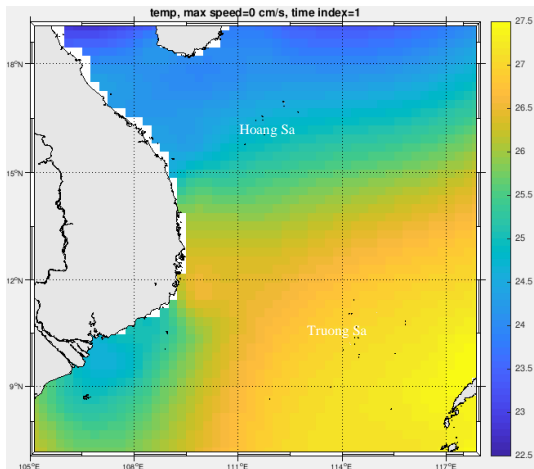
Fig. 3. Temperature initial condition
