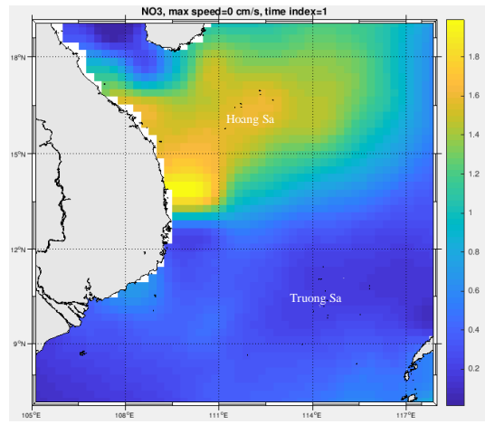
Fig. 6. NO 3 concentration initial condition
