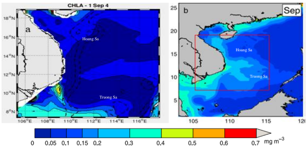
Fig. 20. Comparison of average chlorophyll concentration in September between: (a) this study's result and (b) Peng Xiu's result [10]
