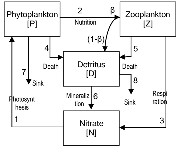
Fig. 1. Diagram of nitrogen cycle (NPZD model [4])
