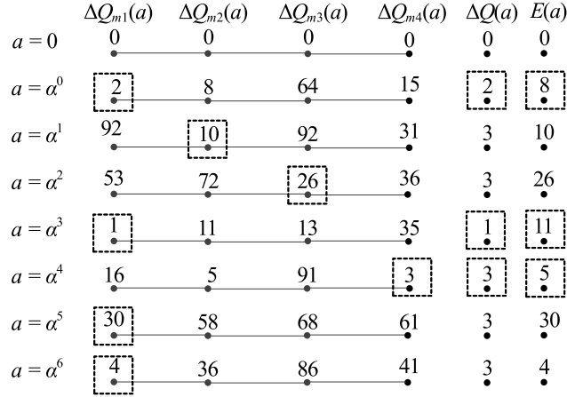
Figure 1. Example of the trellis based on GF(8) with d_c = 4
