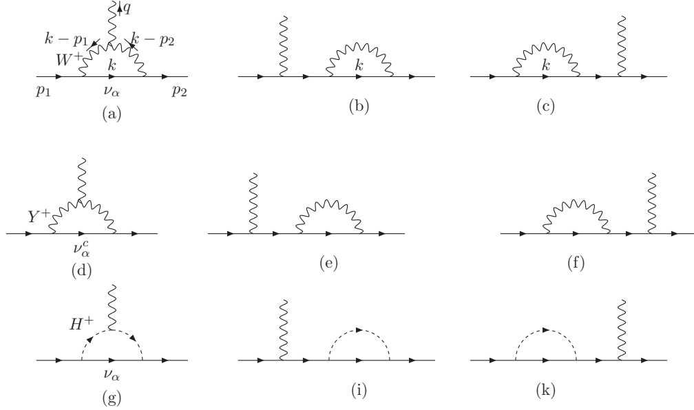
Fig. 1. One-loop Feynman diagrams contribute to l_1 \rightarrow l_2 \gamma in the unitary gauge
