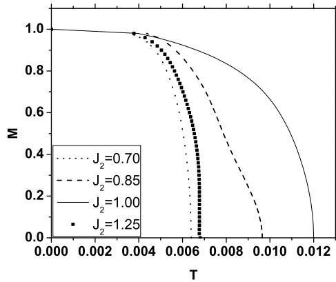
Fig. 1. Temperature dependent magnetization for various J_2/J_1 for W_1 = W_2 = J_1 = 1 and n = 0.025 , x = 0.05 .
