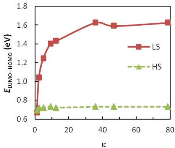
Fig. 6. The \varepsilon dependence of the HOMO-LUMO gap of the LS and HS states of [\text{Fe}^{2+}] molecule.
