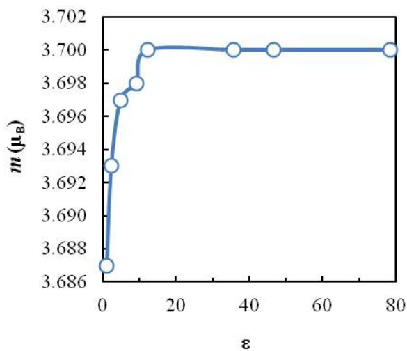
Fig. 5. The \epsilon dependence of the magnetic moment of Fe atom in the HS state of [\text{Fe}^{2+}] molecule.
