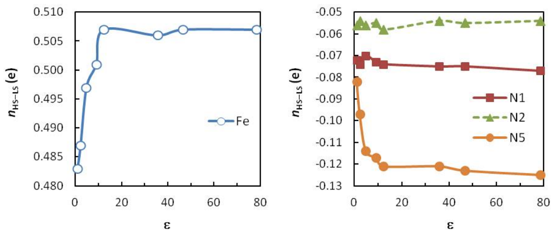
Fig. 4. Influence of solvents on the charge transfer upon crossover from the LS state to the HS state of [\text{Fe}^{2+}] molecule.
