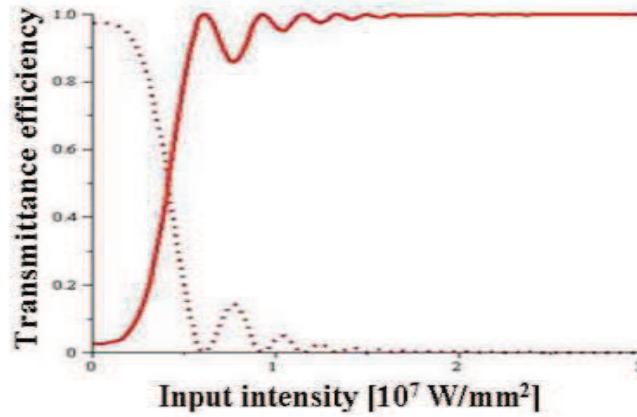
Fig. 2. The transfer efficiency through linear output port (solid) and nonlinear output port (dot) of NOC with n_{nl} = 1.0 \times 10^{-12} \text{ mm}^2/\text{W} , l_{cpl} = 2.5 \text{ mm} vs input intensity density at \lambda = 1.5 \mu\text{m} .
