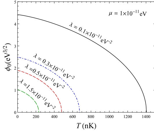
Fig. 3. The T dependence of order parameter \phi_0 at \mu = 10^{-11} \text{ eV} and several values of \lambda
