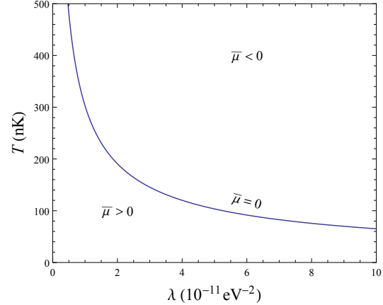
Fig. 6. Phase diagram of restoration transition in the (T, \lambda) - plane. The broken phase ( \bar{\mu} > 0 ) and unbroken phase ( \bar{\mu} < 0 ) are separated by the phase diagram ( \bar{\mu} = 0 )
