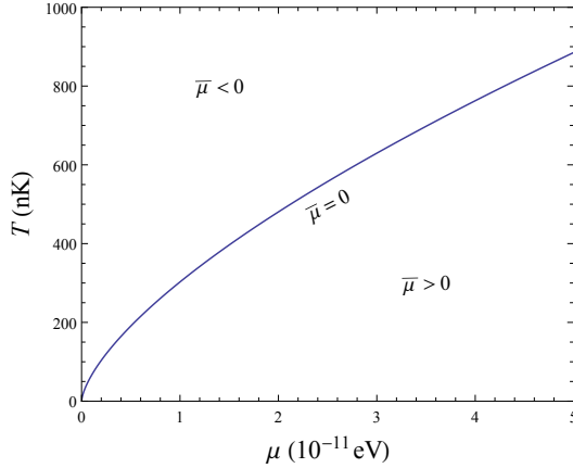
Fig. 5. Phase diagram of restoration transition in the (T, \mu) - plane. The broken phase ( \bar{\mu} > 0 ) and unbroken phase ( \bar{\mu} < 0 ) are separated by the phase diagram ( \bar{\mu} = 0 )
