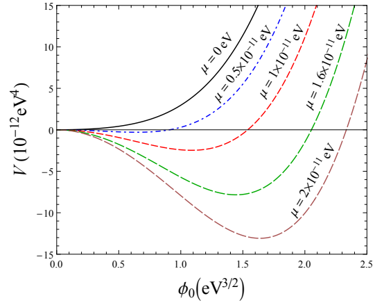
Fig. 2. The evolution of effective potential V against \phi_0 at \lambda = 10^{-11} \text{eV}^{-2} and several values of \mu
