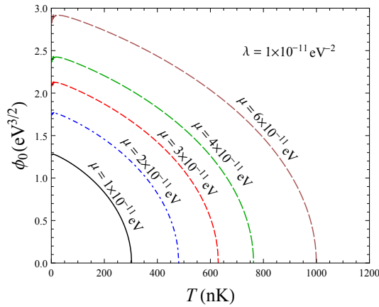
Fig. 1. The T dependence of order parameter \phi_0 at \lambda = 10^{-11} \text{eV}^{-2} and several values of \mu
