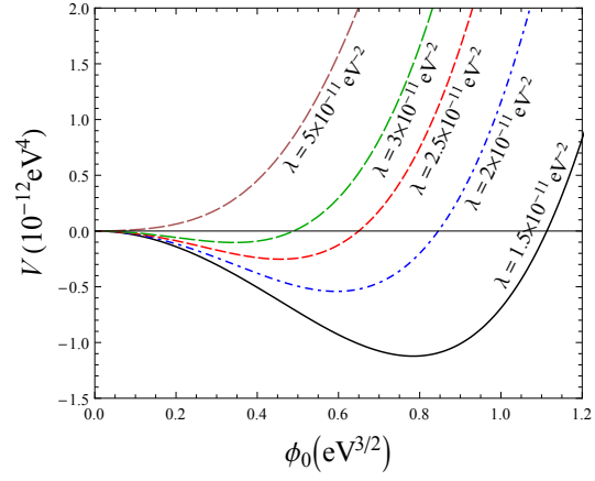
Fig. 4. The evolution of effective potential V against \phi_0 at \mu = 10^{-11} \text{ eV} and several values of \lambda
