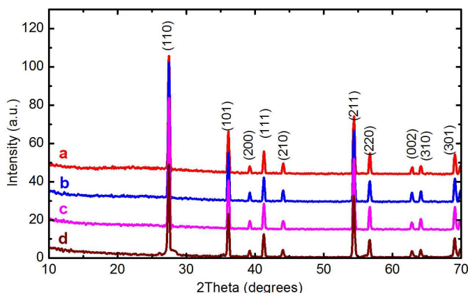
Fig. 6. XRD patterns of the \text{Ti}_{1-x}\text{Cr}_x\text{O}_2 samples with different molar fractions x , heat-treated at 1100 °C for 3 h: a) x = 0.005 , b) x = 0.01 , c) x = 0.04 and d) x = 0.1 .
