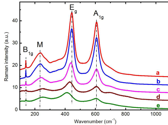
Fig. 8. Raman spectra of the rutile \text{Ti}_{1-x}\text{Cr}_x\text{O}_2 samples with different molar fractions x , heat-treated at 1100^\circ\text{C} for 3 h: a) x = 0 , b) x = 0.005 , c) x = 0.01 and d) x = 0.08 .
