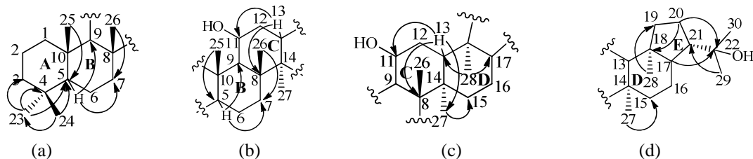
(a) A/B ring fusion in fragment 1 (c) C/D ring fusion in fragment 3 (b) B/C ring fusion in fragment 2 (d) D/E ring fusion in fragment 4
